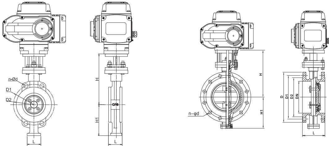
对夹连接 主要外形及连接尺寸 GB-PN16(1.6MPa) Wafer Type Main Outline and Connecting Size
